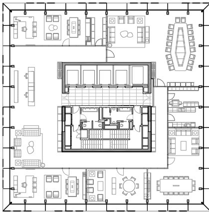
PLANTA 21 / 21ND FLOOR PLAN
