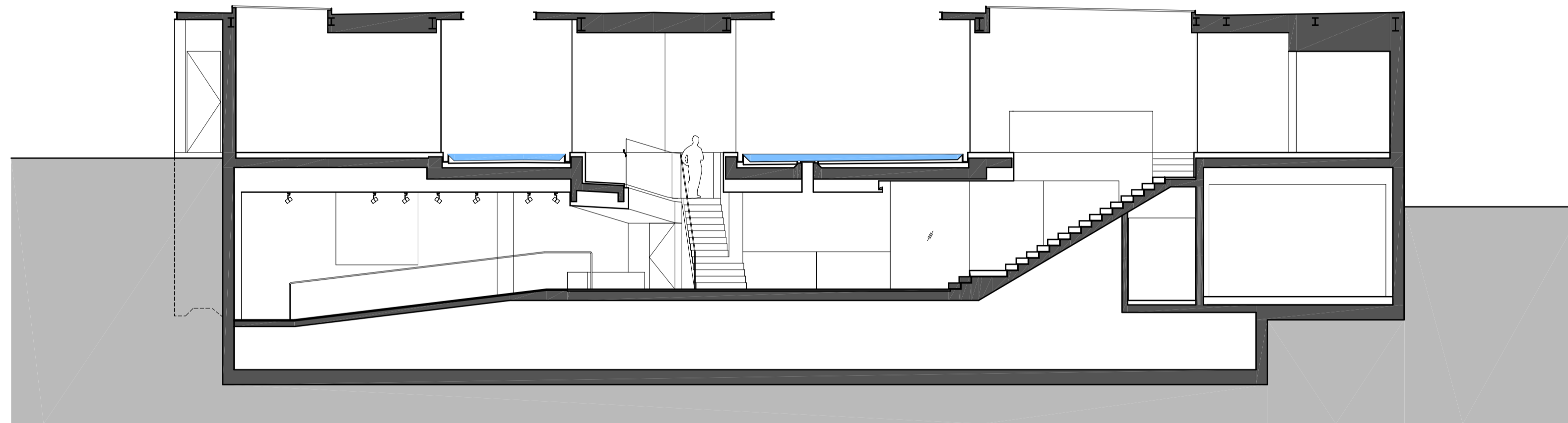
SECTION B-B
