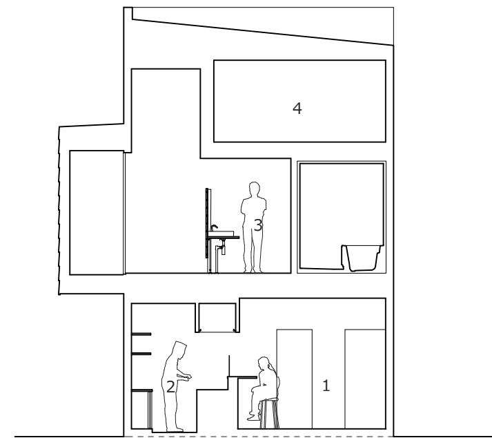
sectional view 1:100
