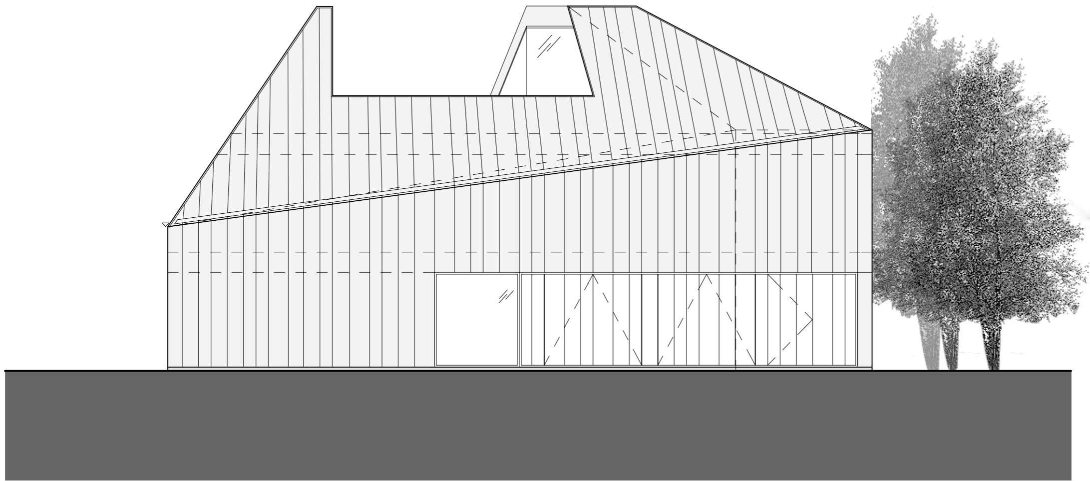
South elevation
