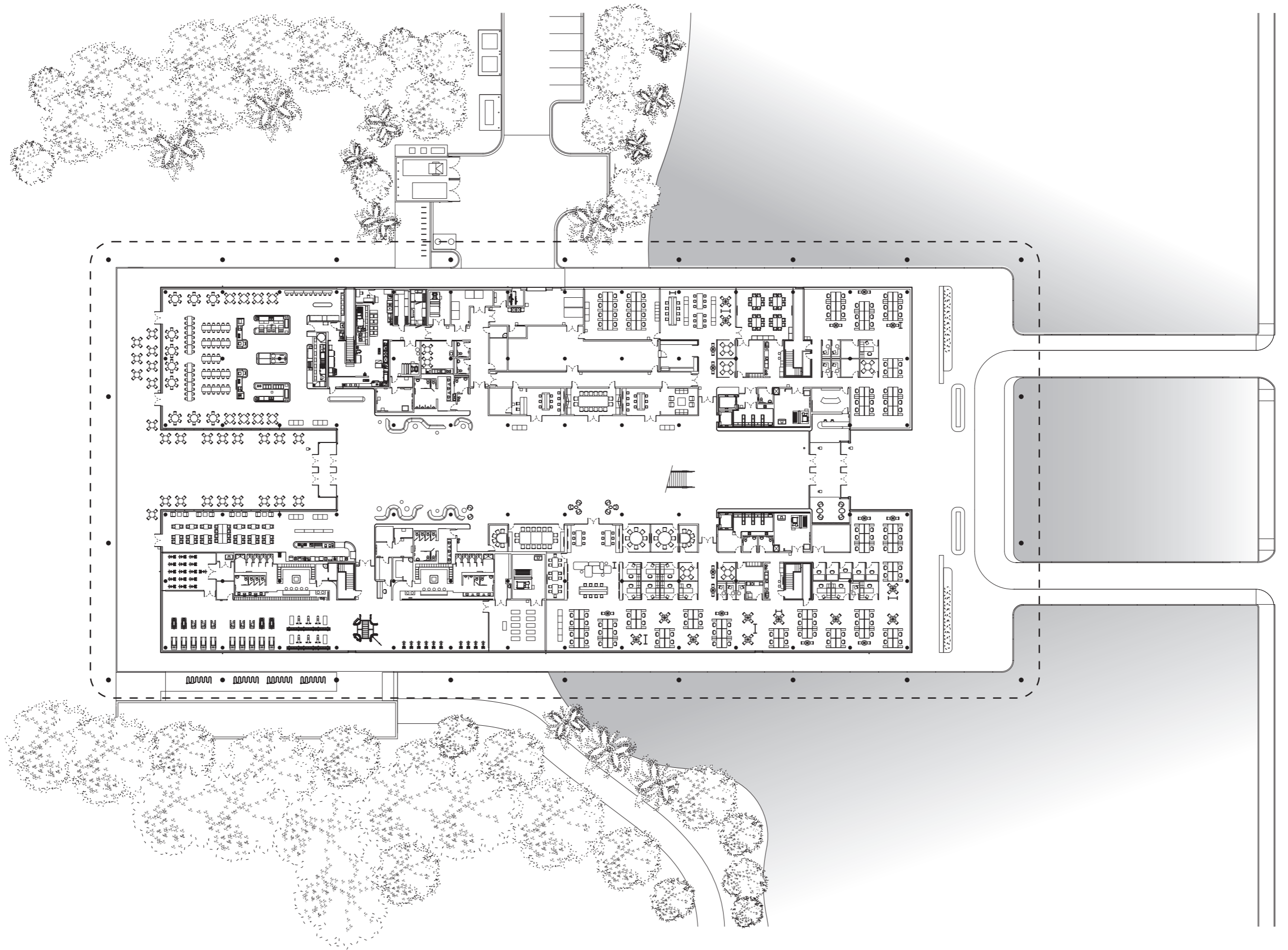
Floor Plan - Level 1
