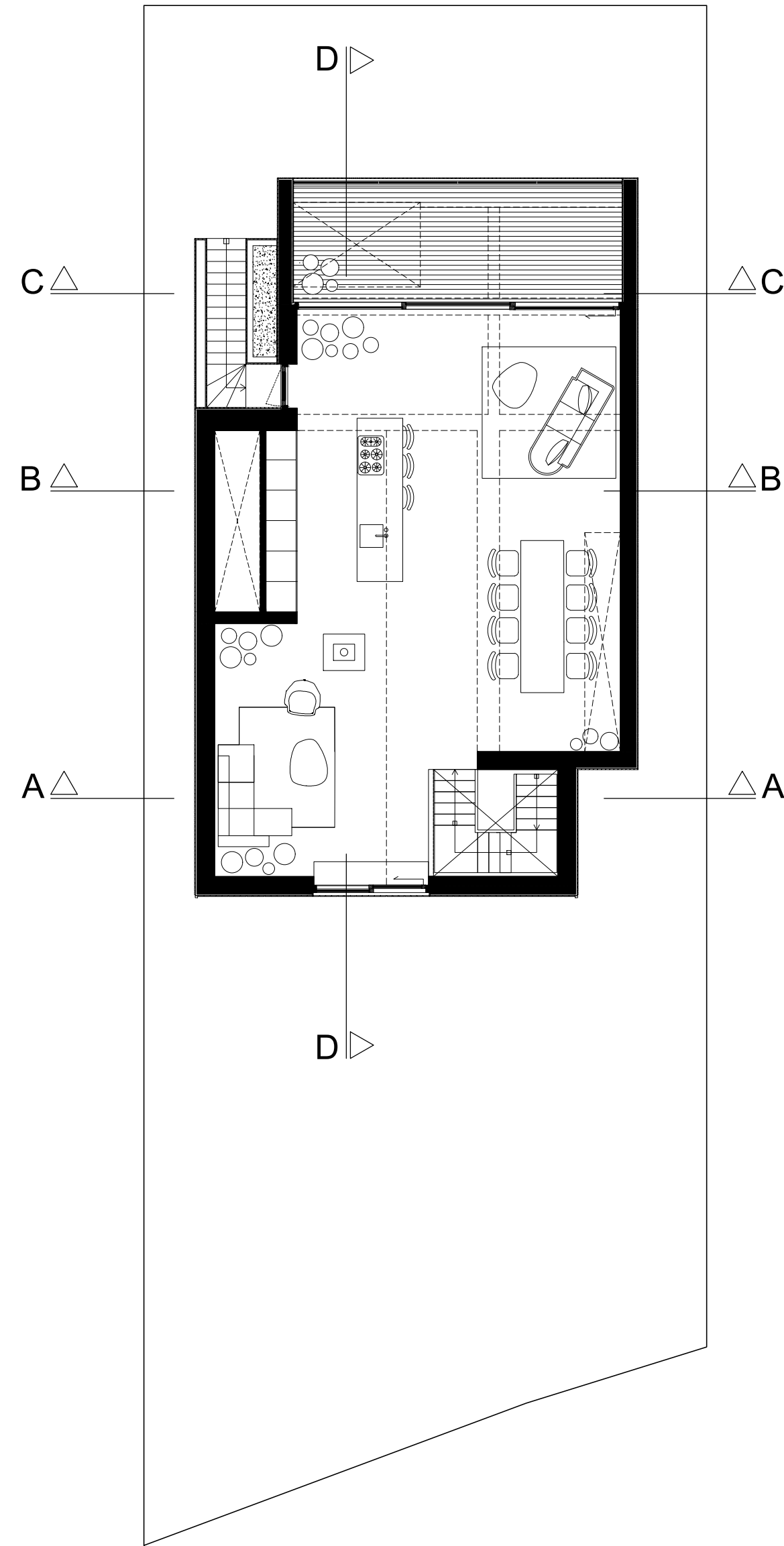
FIRST FLOOR
