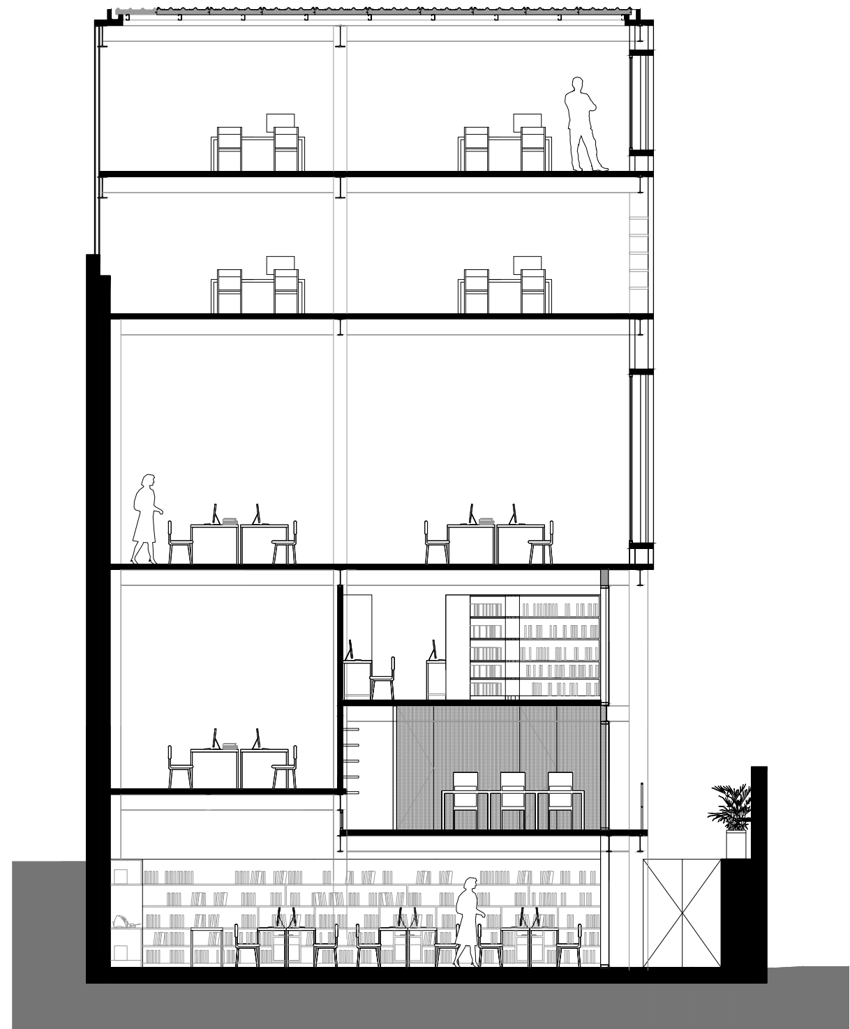
Section 4-4' Havre 77
