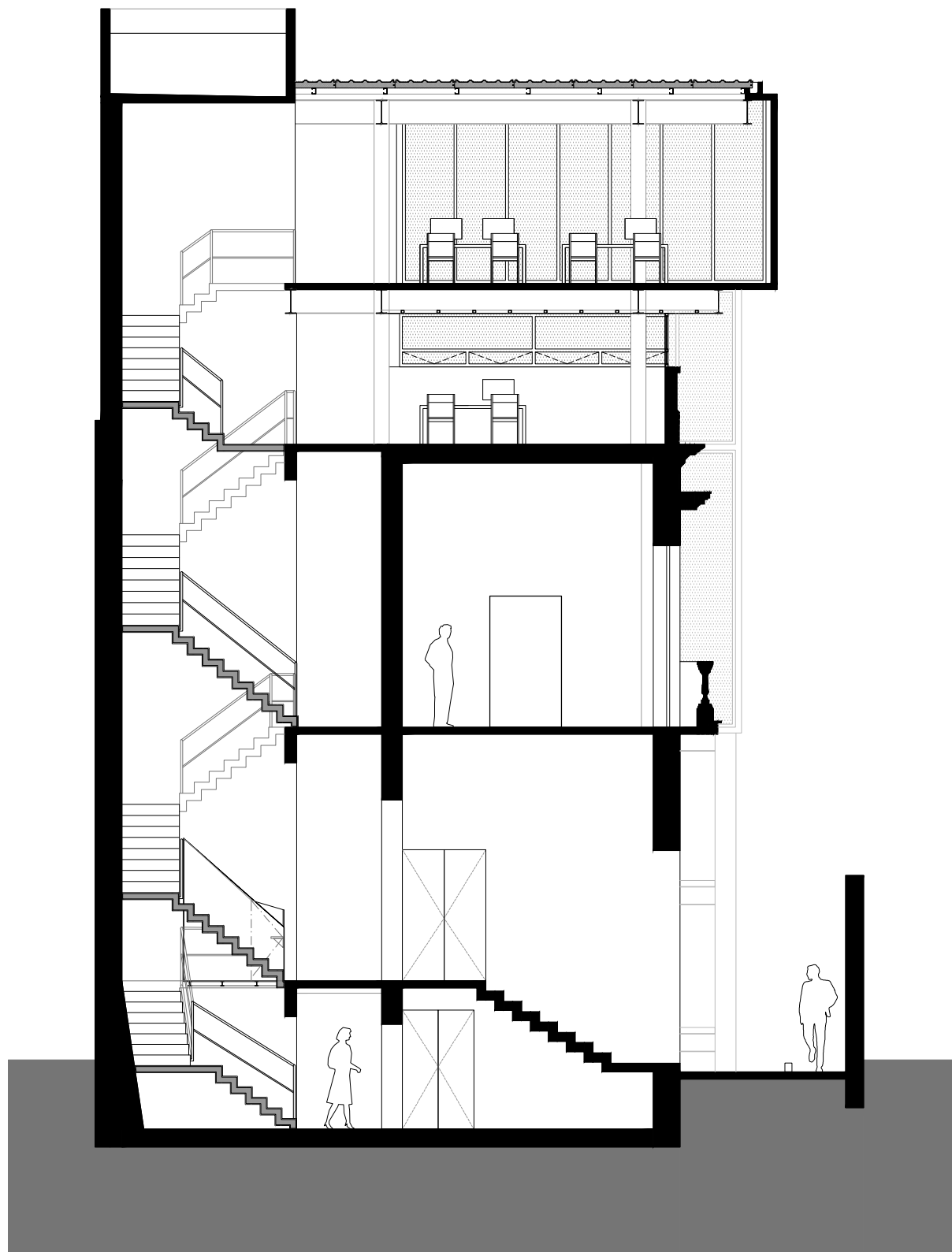
Section 2-2' Havre 77
