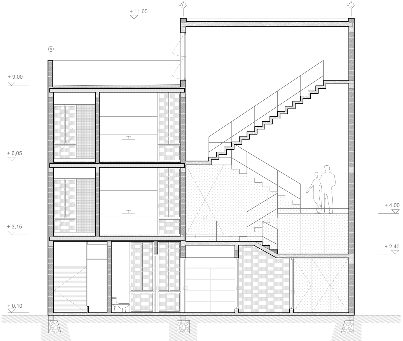
SECTION S3
