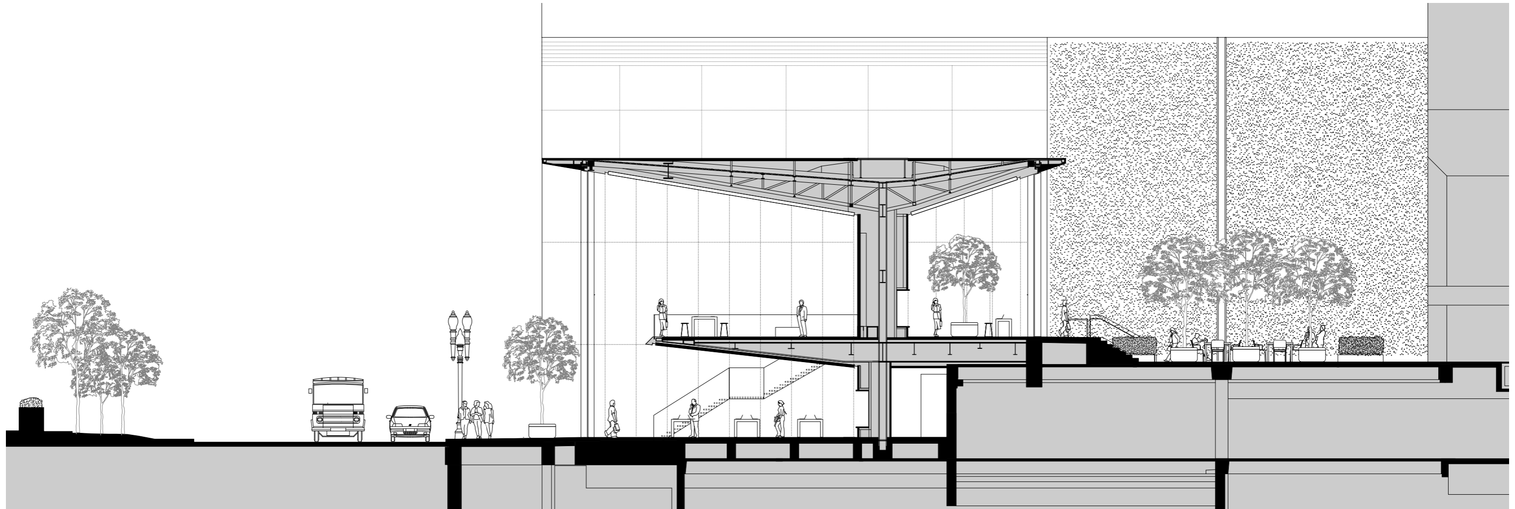
Long Section - Store
