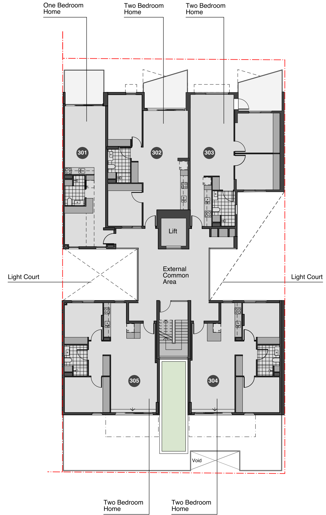
Third Level Floor Plan 1:200 @A3
