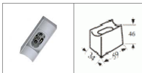
OSRAM Linestra Fass 662 Cap s14S mm. 34 x 59 x 46
