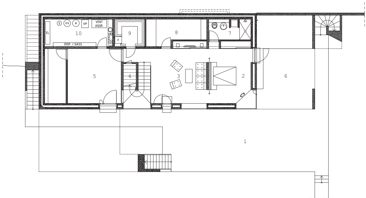
GROUND FLOOR PLAN 1:200/A4
