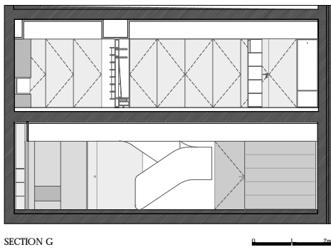
SECTION G
