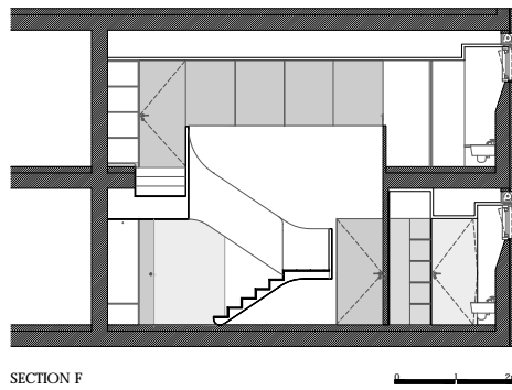
SECTION F
