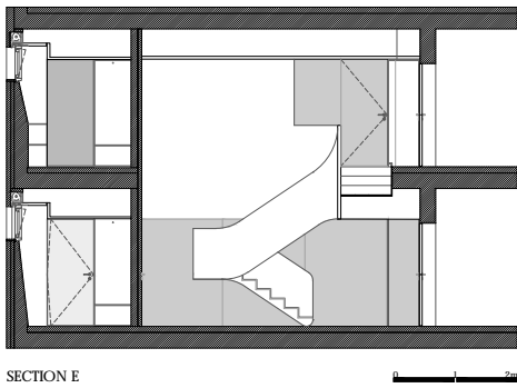
SECTION E
