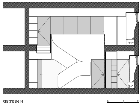
SECTION H
