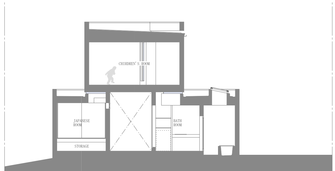
Section B-B' S=1:100
