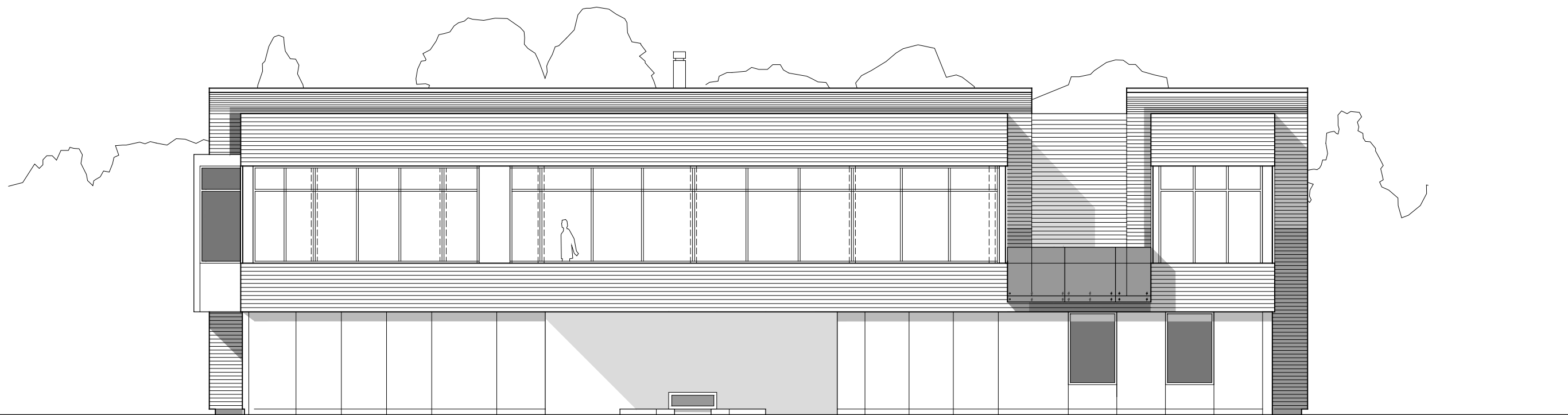
NORTH ELEVATION
