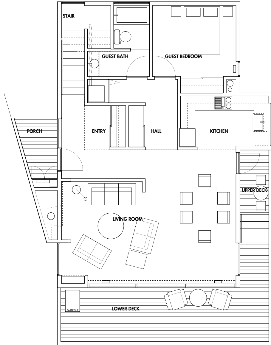
1 FIRST FLOOR PLAN A2.1
