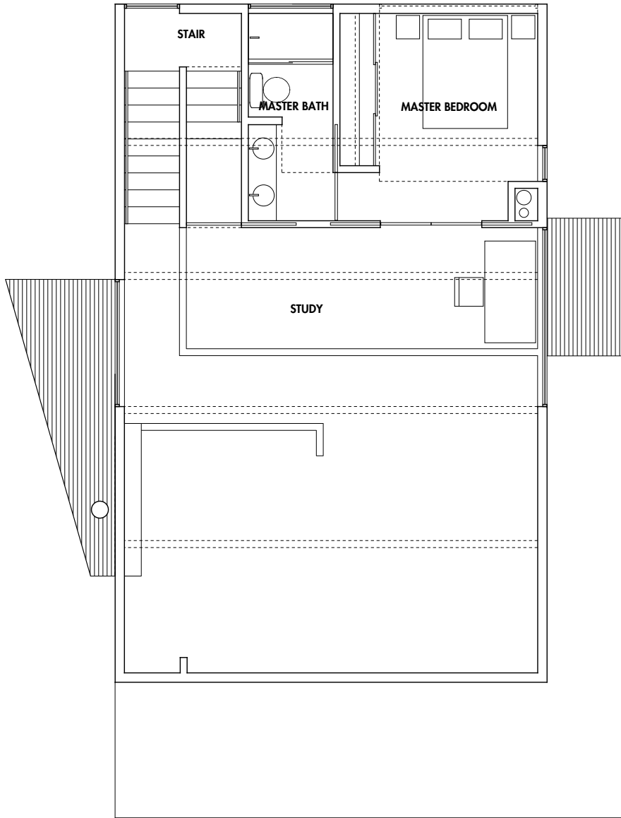
2 SECOND FLOOR PLAN A2.1
