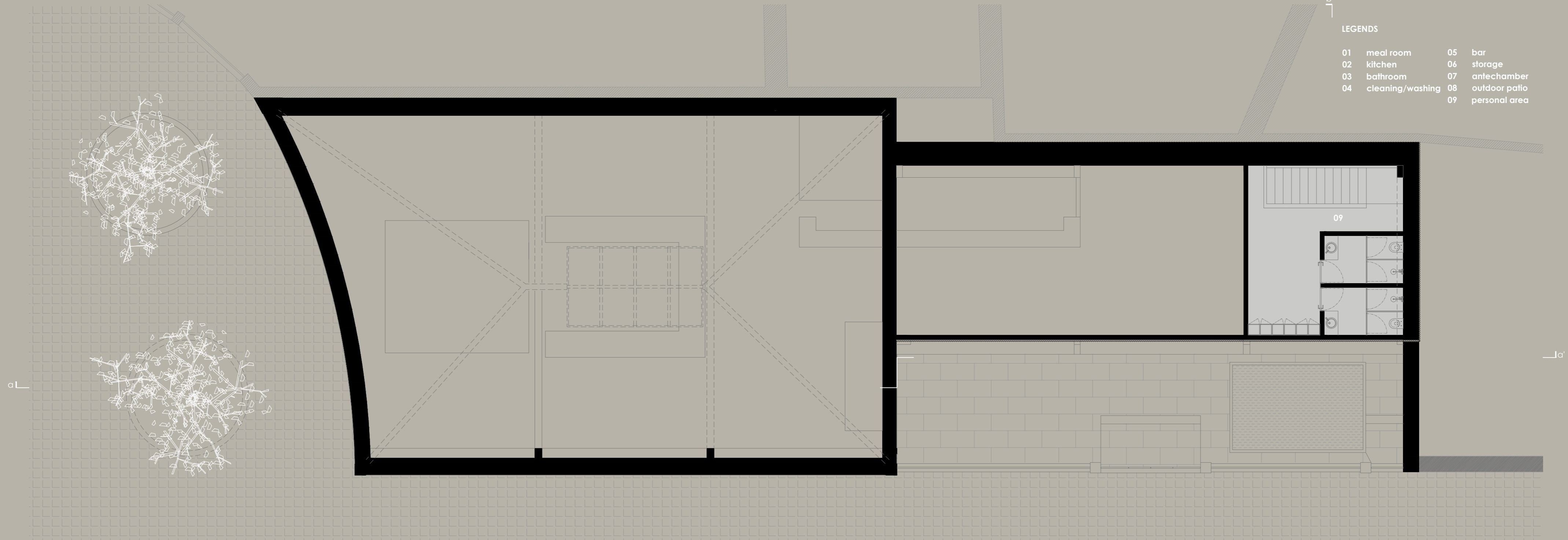
floor plan 1
