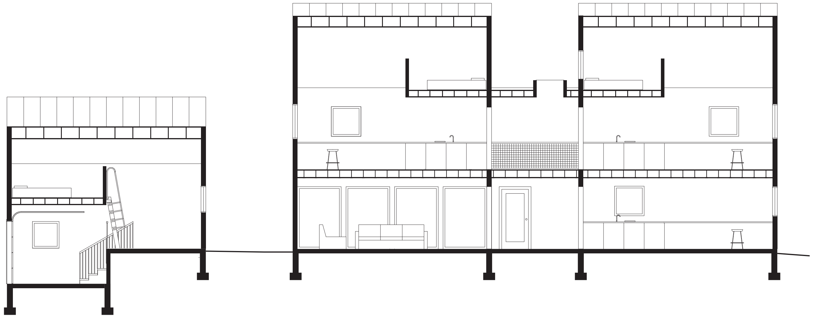
CORTE 2-2'
