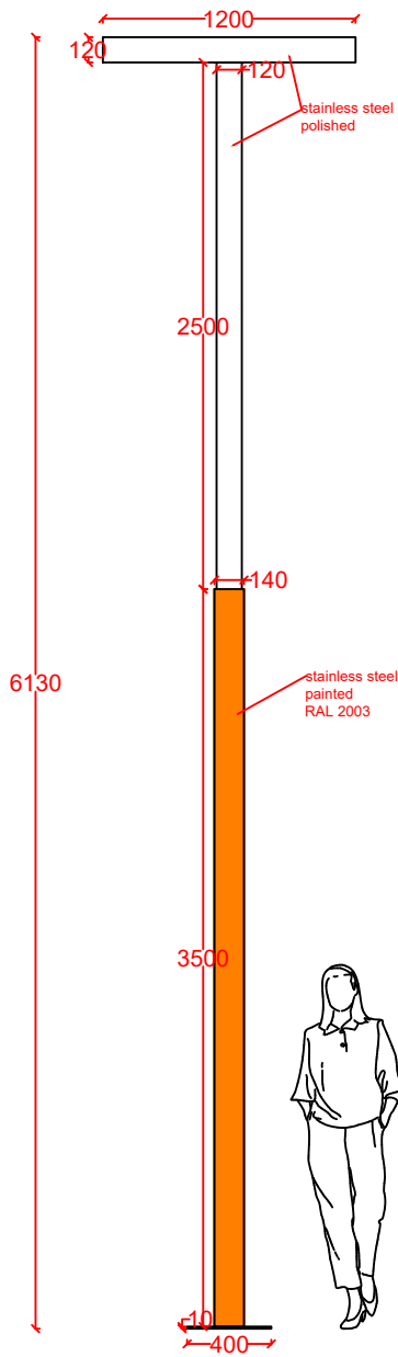
Front view
