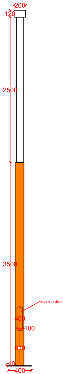
Side view
