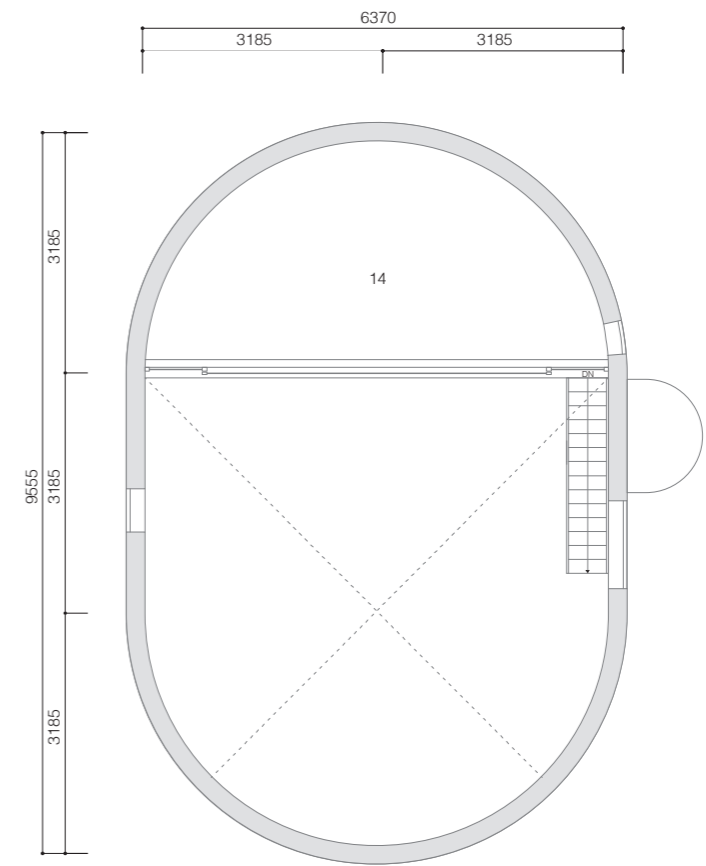
terrace level plan 1:100
