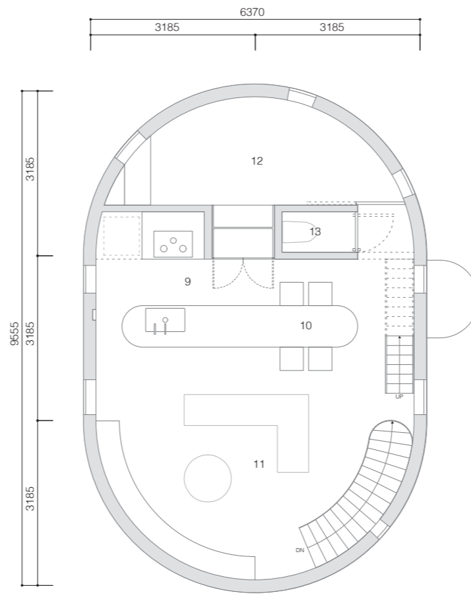
2F plan 1:100
