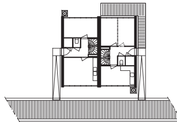
laag 00
