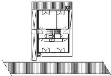
laag 00
