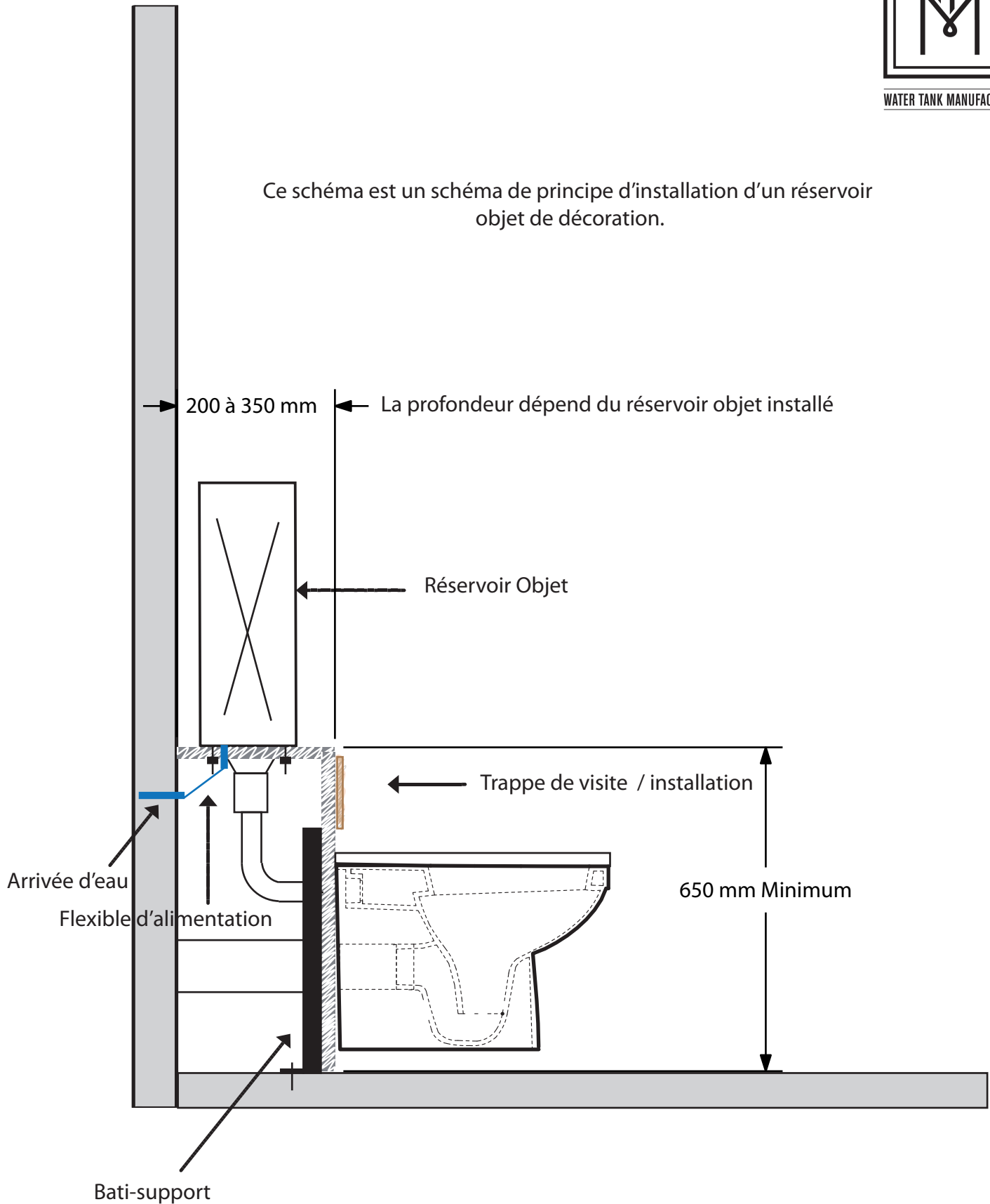
SIDE VIEW WTKM ROBJETS INSTALLATION
