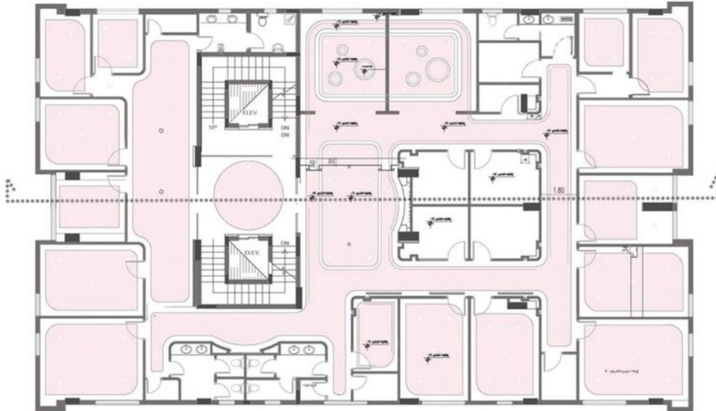
ceiling plan
