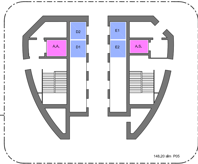
Diagram 3: Elevator Configuration CityLife_Generali Tower
