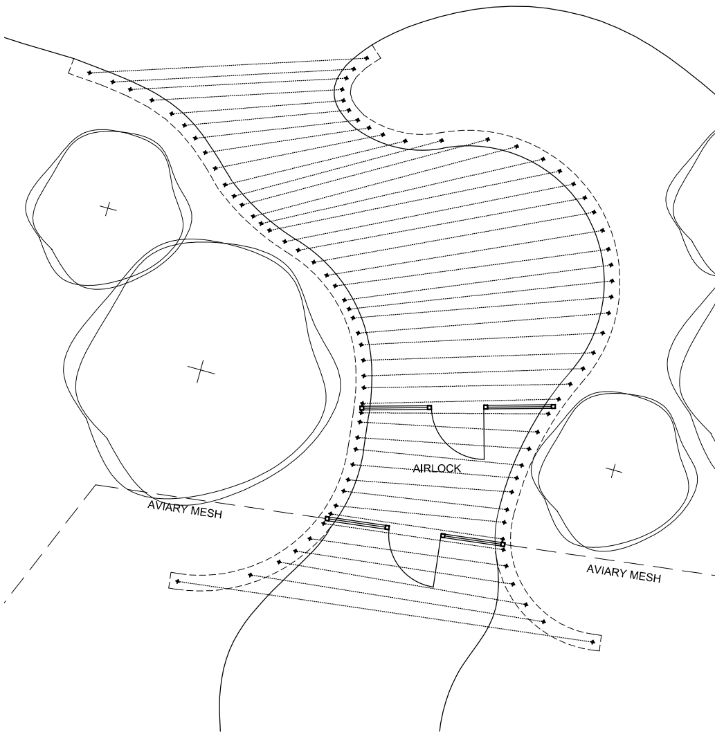
ENTRY TUNNEL FLOORPLAN
