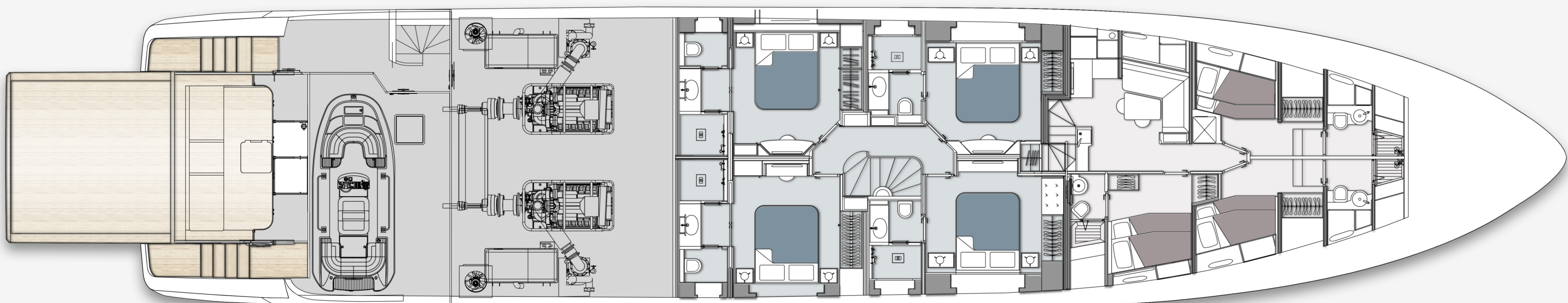
LOWER DECK
