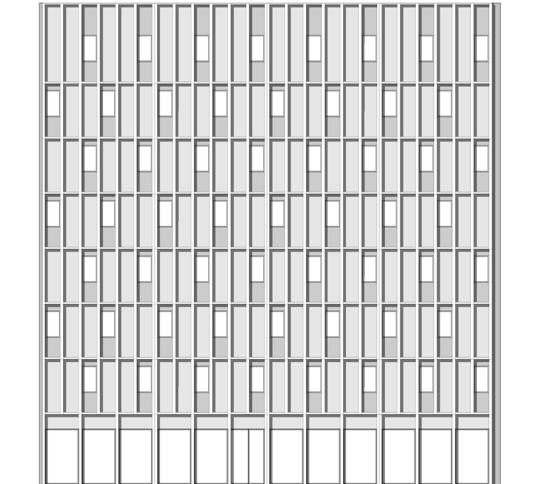
STREET ELEVATION
