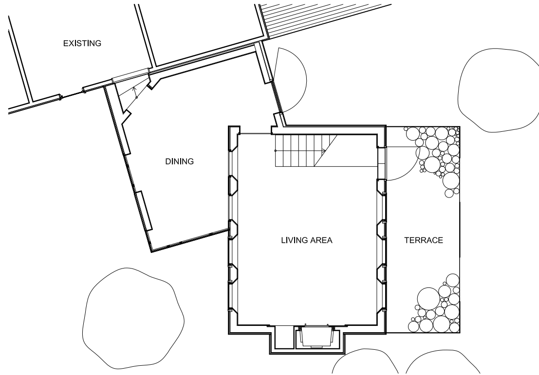
GF PLAN 1:100
