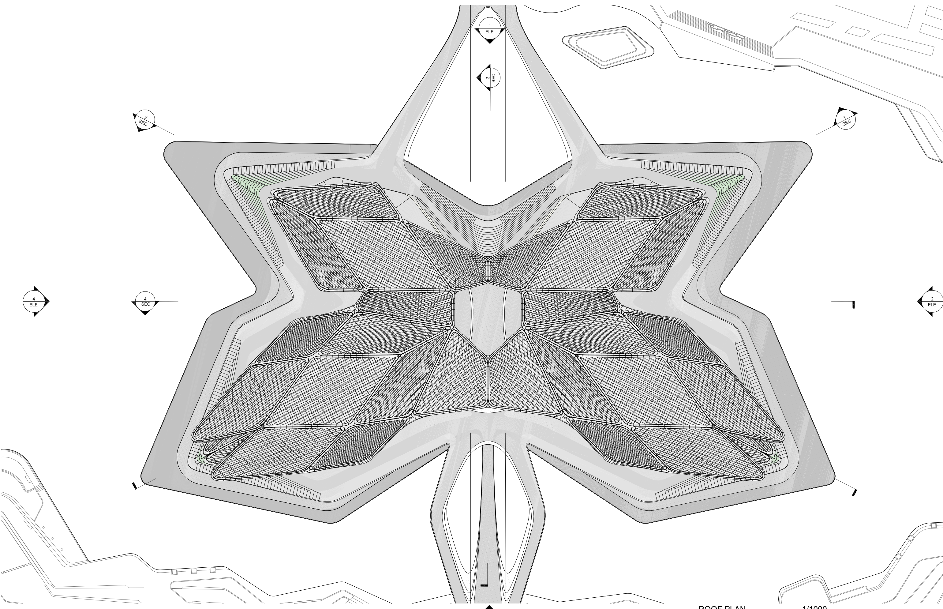
ROOF PLAN 1/1000 0 10 20 50 80m N
