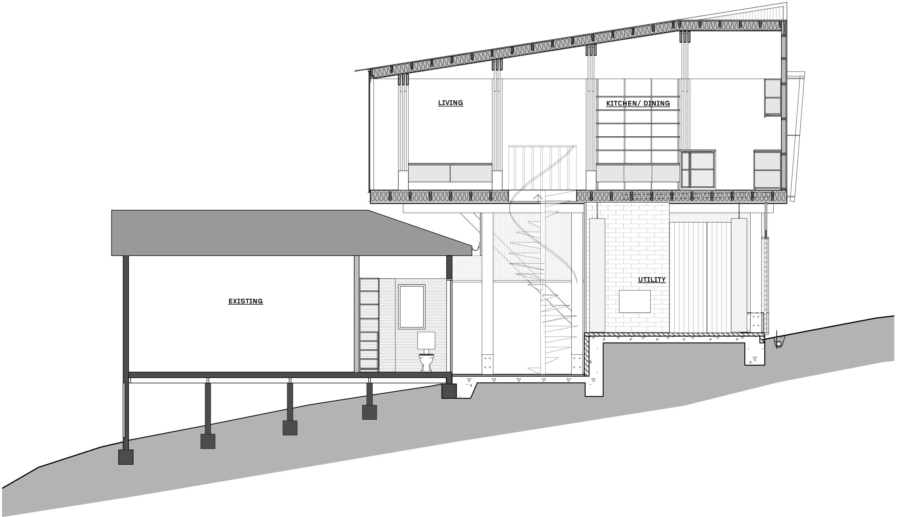
Section 1:50
