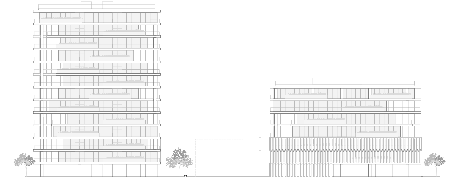
Alzado Noroeste. Northwest Elevation
