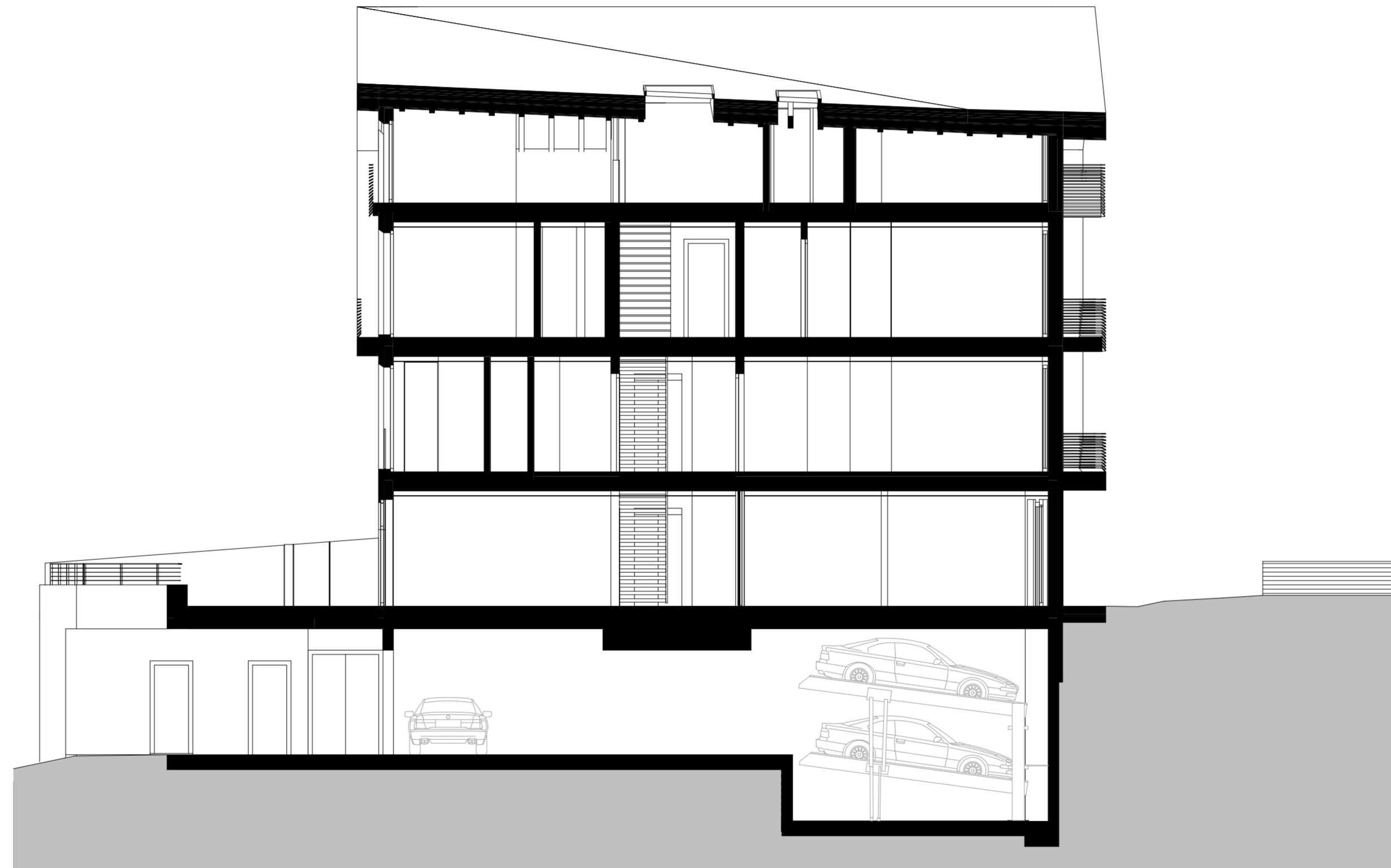
Section B-B S 1:100
