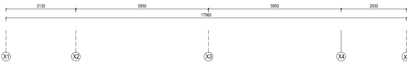
ROOF PLAN
