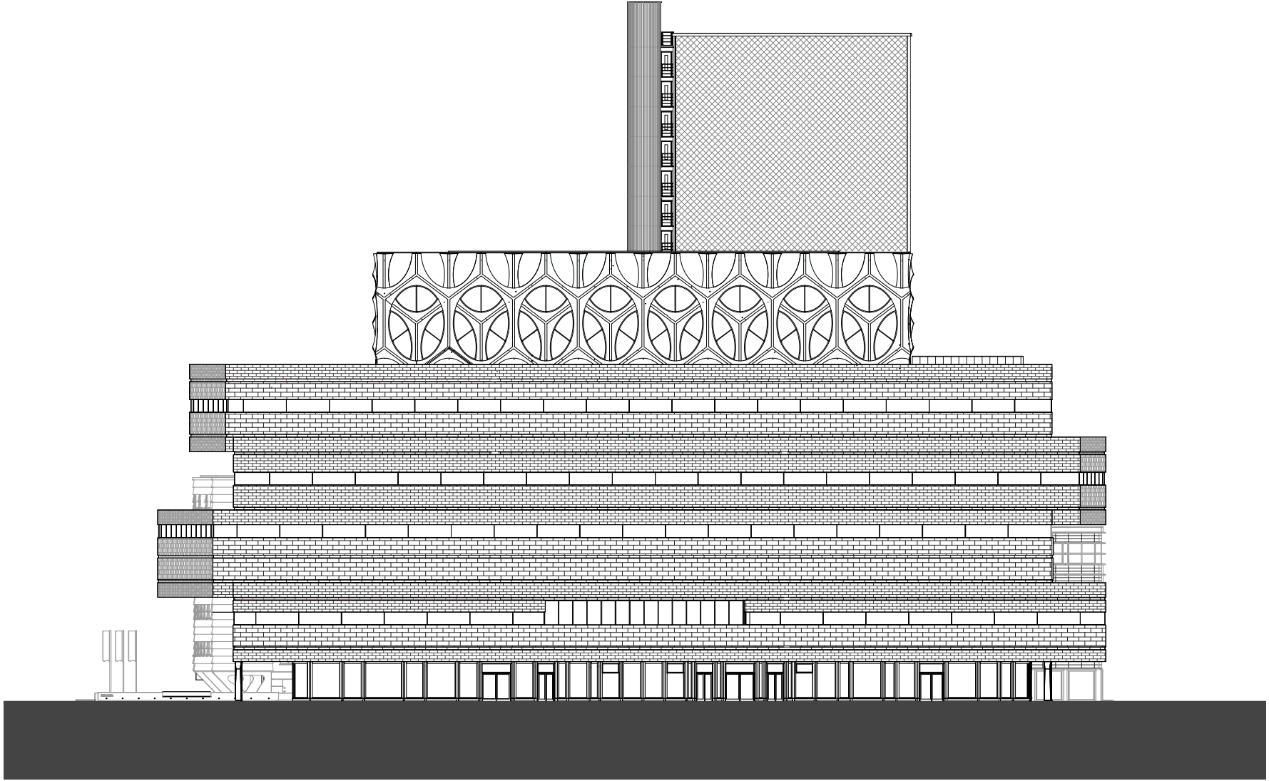
North facade
