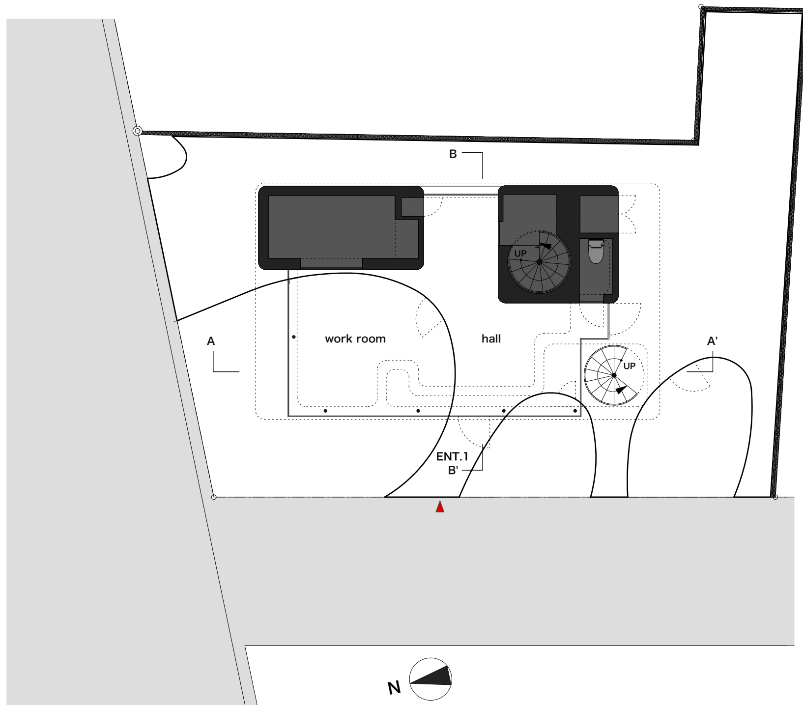
1st floor plan S=1:100
