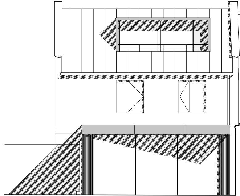
Rear Elevation
