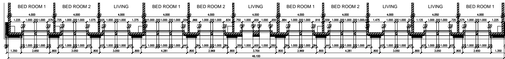
FIRST FLOOR LEVEL (SIDE-1)
