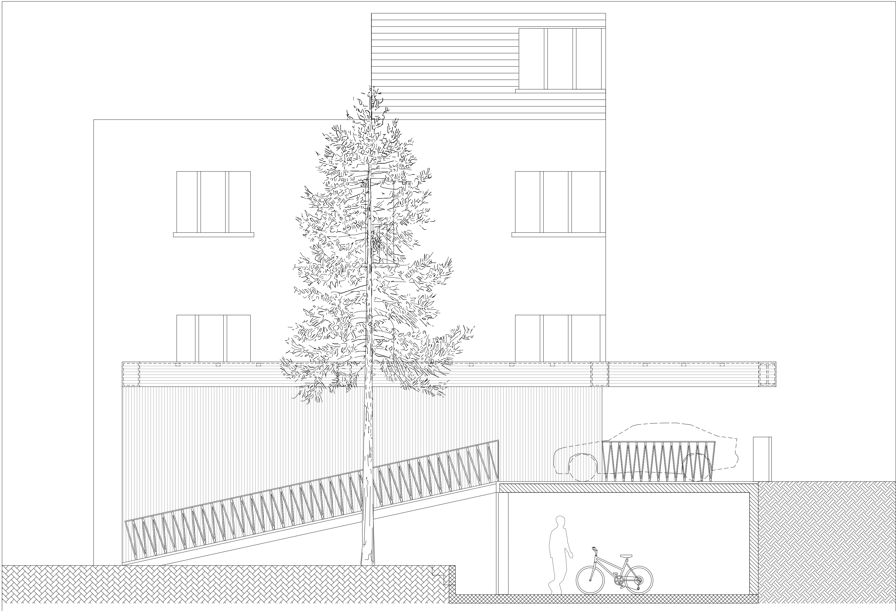
SOUTH VIEW 0 1 2 m
