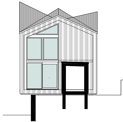
NORTH FACADE
