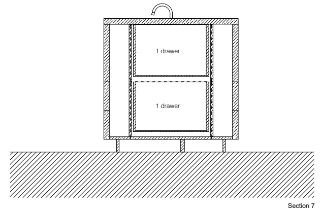
TEA COUNTER DETAILS
