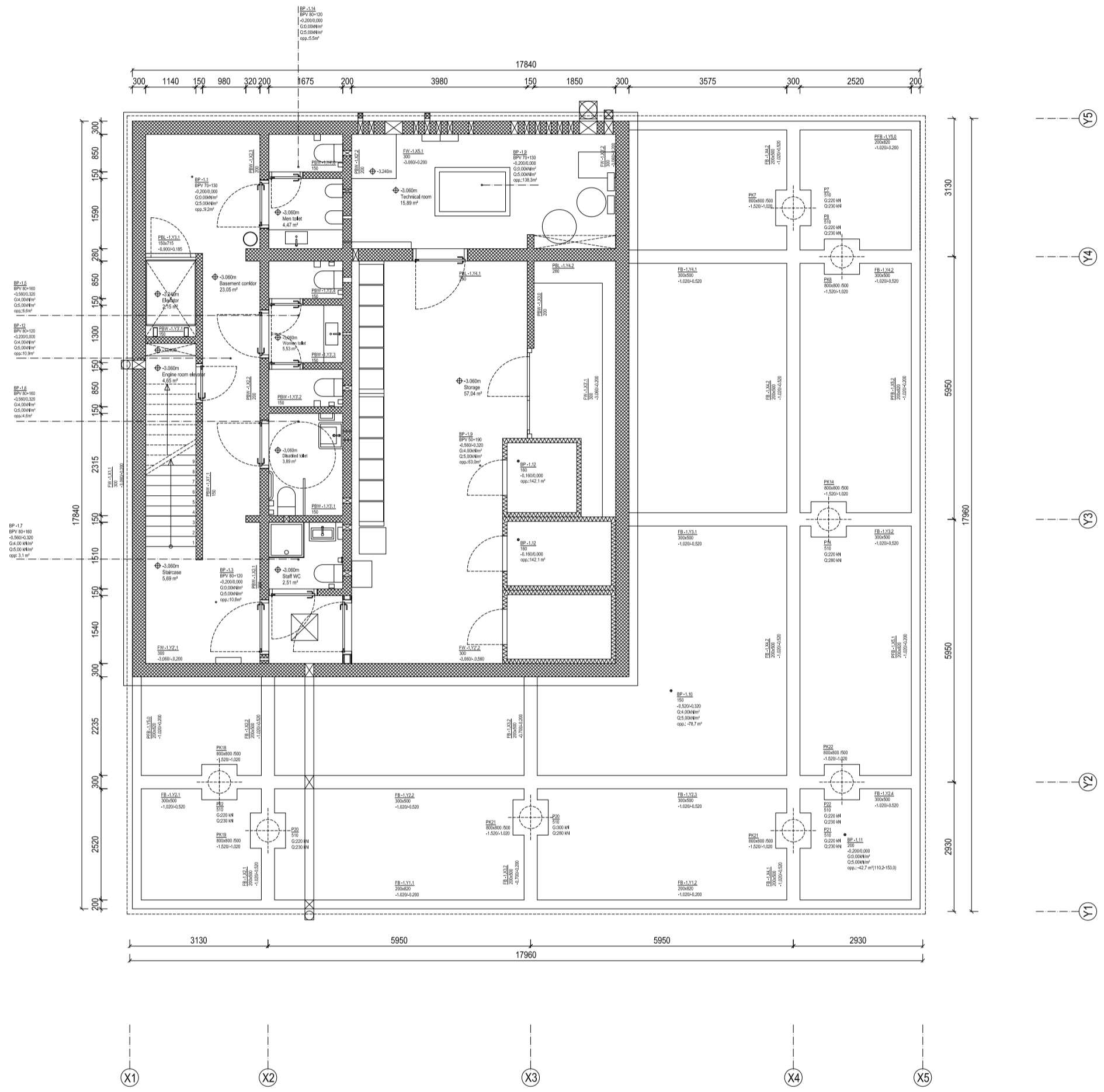
BASEMENT TECHNICAL PLAN
