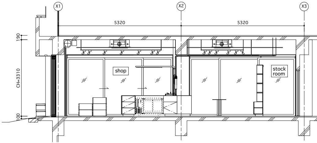
section 1/100
