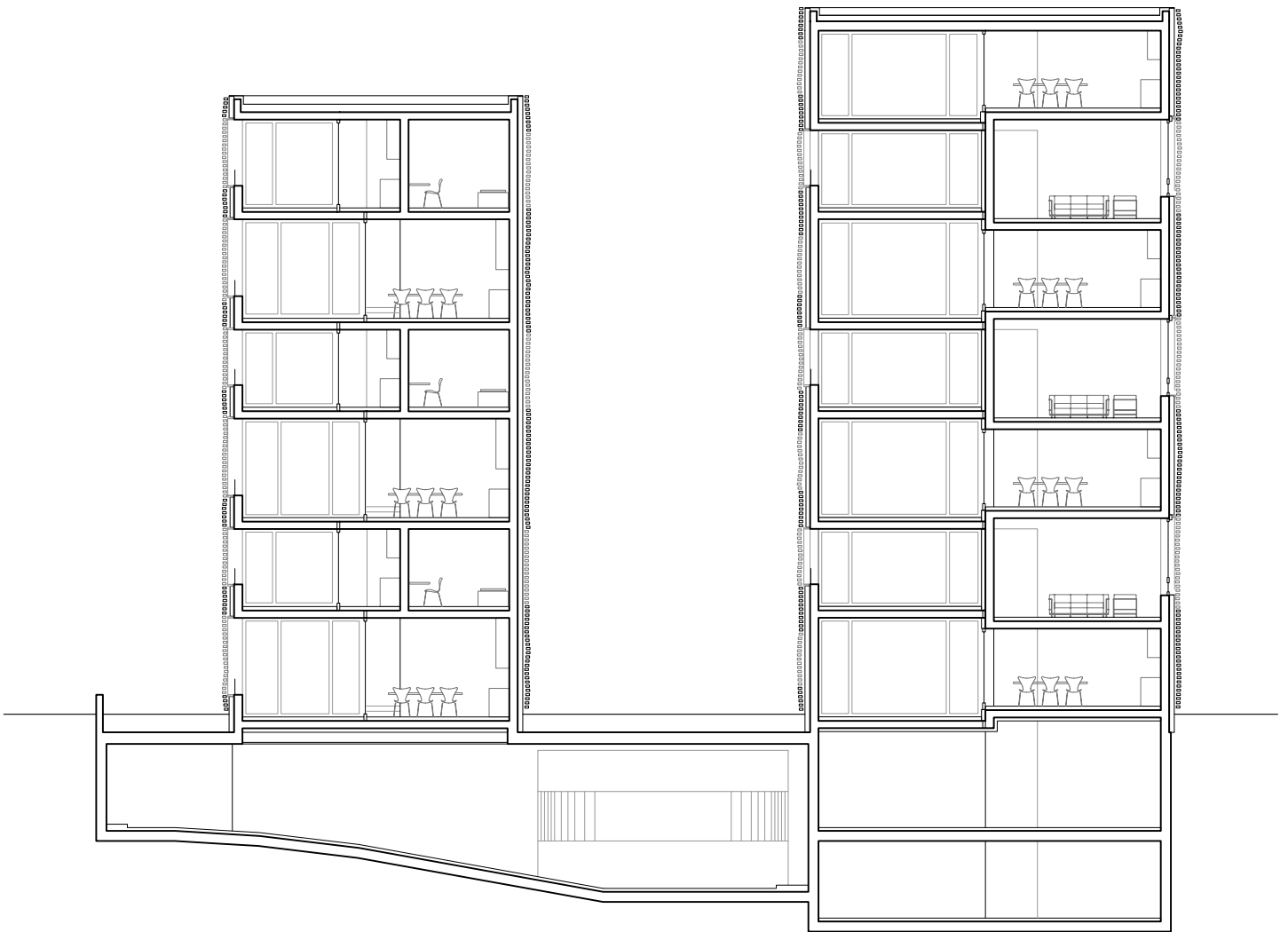
Cross section _ building B and C 1:200
