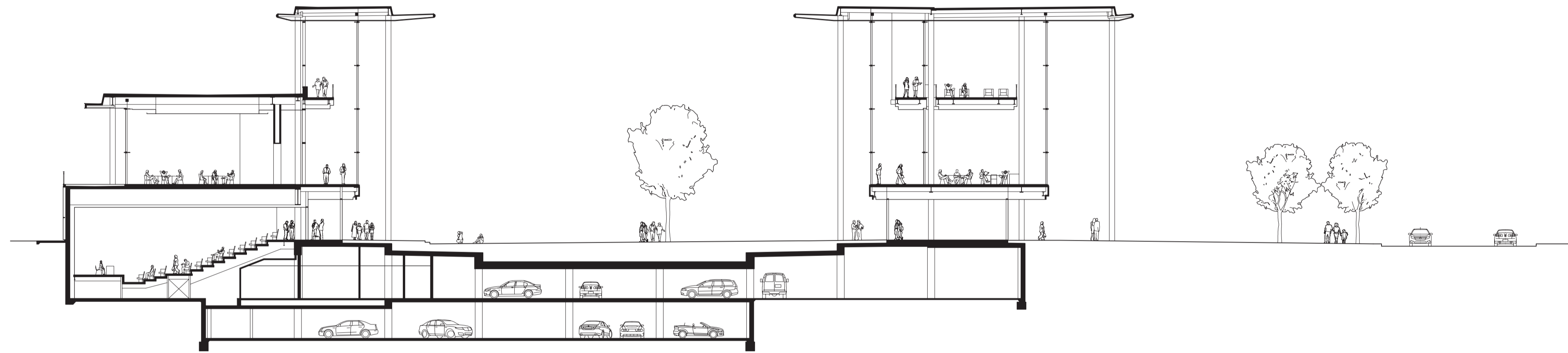
Yale School of Management Cross-section 0 5 10m
