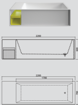
wanna / bathtub #021327
