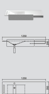
umywalka / washbasin #021222
