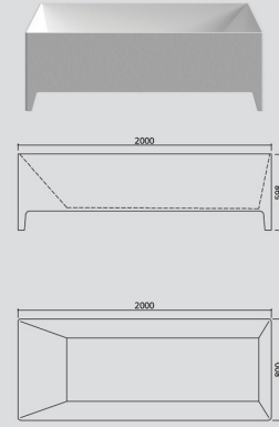
wanna / bathtub #021125
