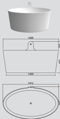
wanna / bathtub #023128
