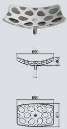
umywalka / washbasin #024322
