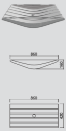
umywalka / washbasin #024221
