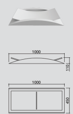
umywalka / washbasin #026121
