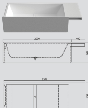
wanna / bathtub #021227
