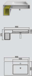
umywalka / washbasin #021322
