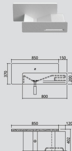
umywalka / washbasin #021223
