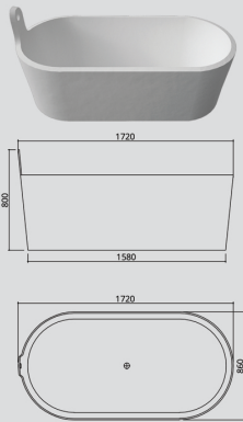
wanna / bathtub #023127
