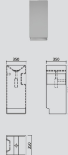
umywalka / washbasin #021224
