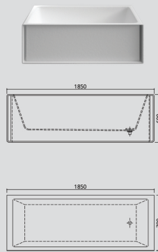
wanna / bathtub #021328
