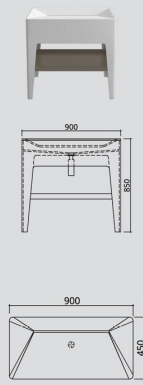
umywalka / washbasin #021122
