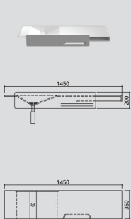
umywalka / washbasin #021221
