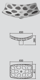
umywalka / washbasin #024321
