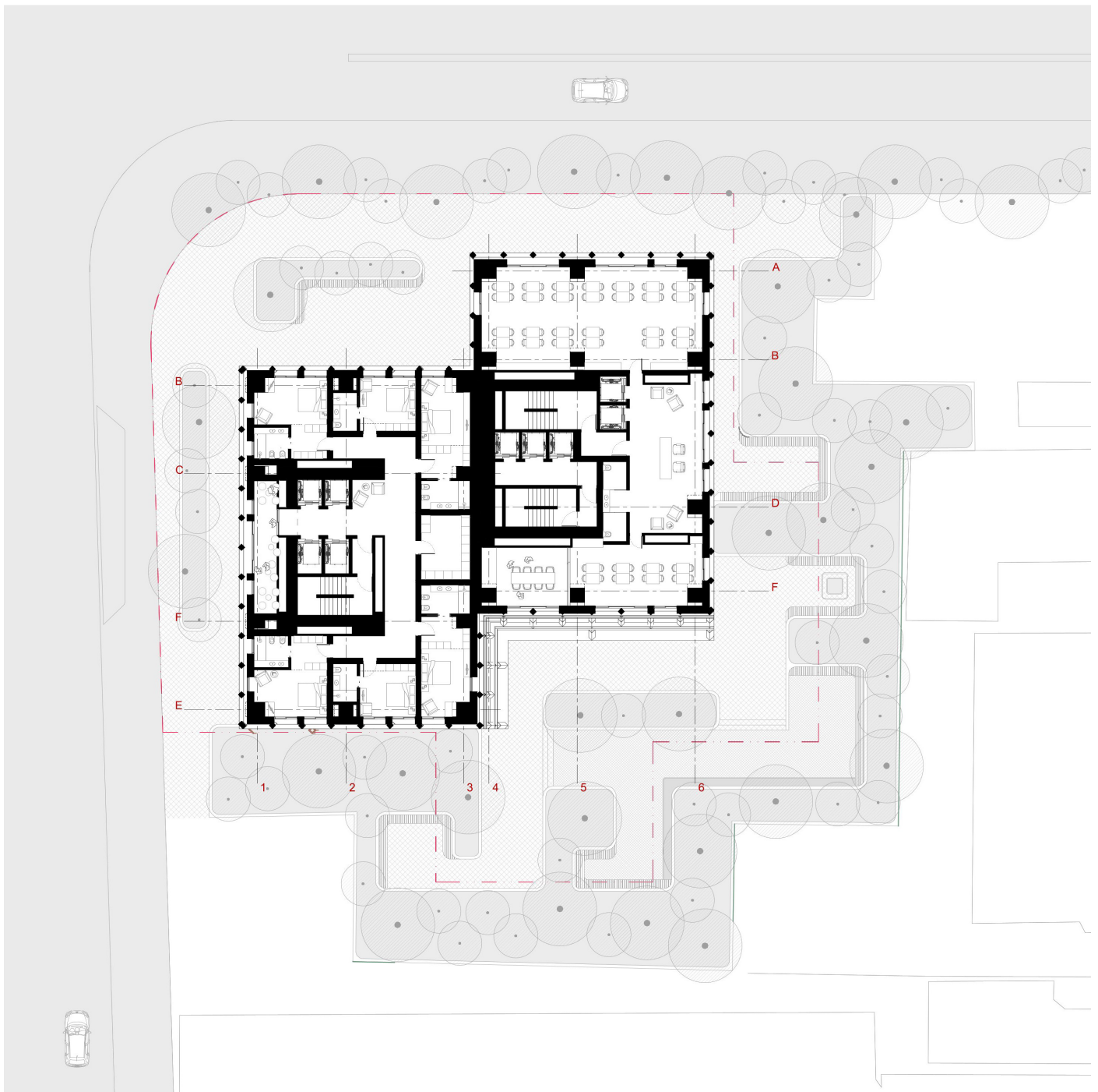
Office and Hotel floor Level plan
