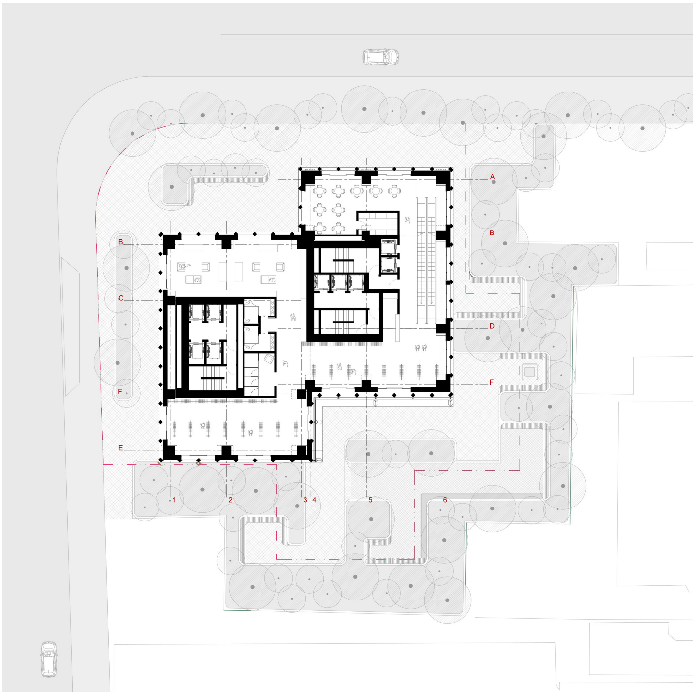
Retail floor Level plan
