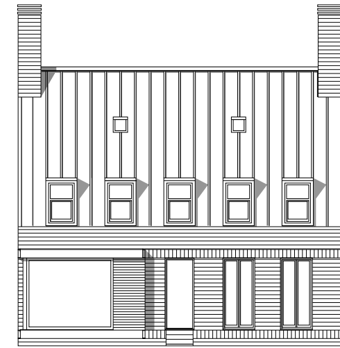
SOUTH FACADE
