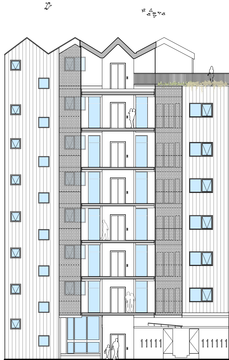
North Light Court Elevation 1:200 @ A3
