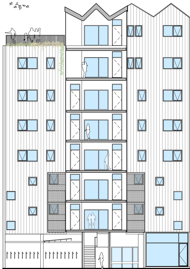
South Light Court Elevation 1:200 @ A3
