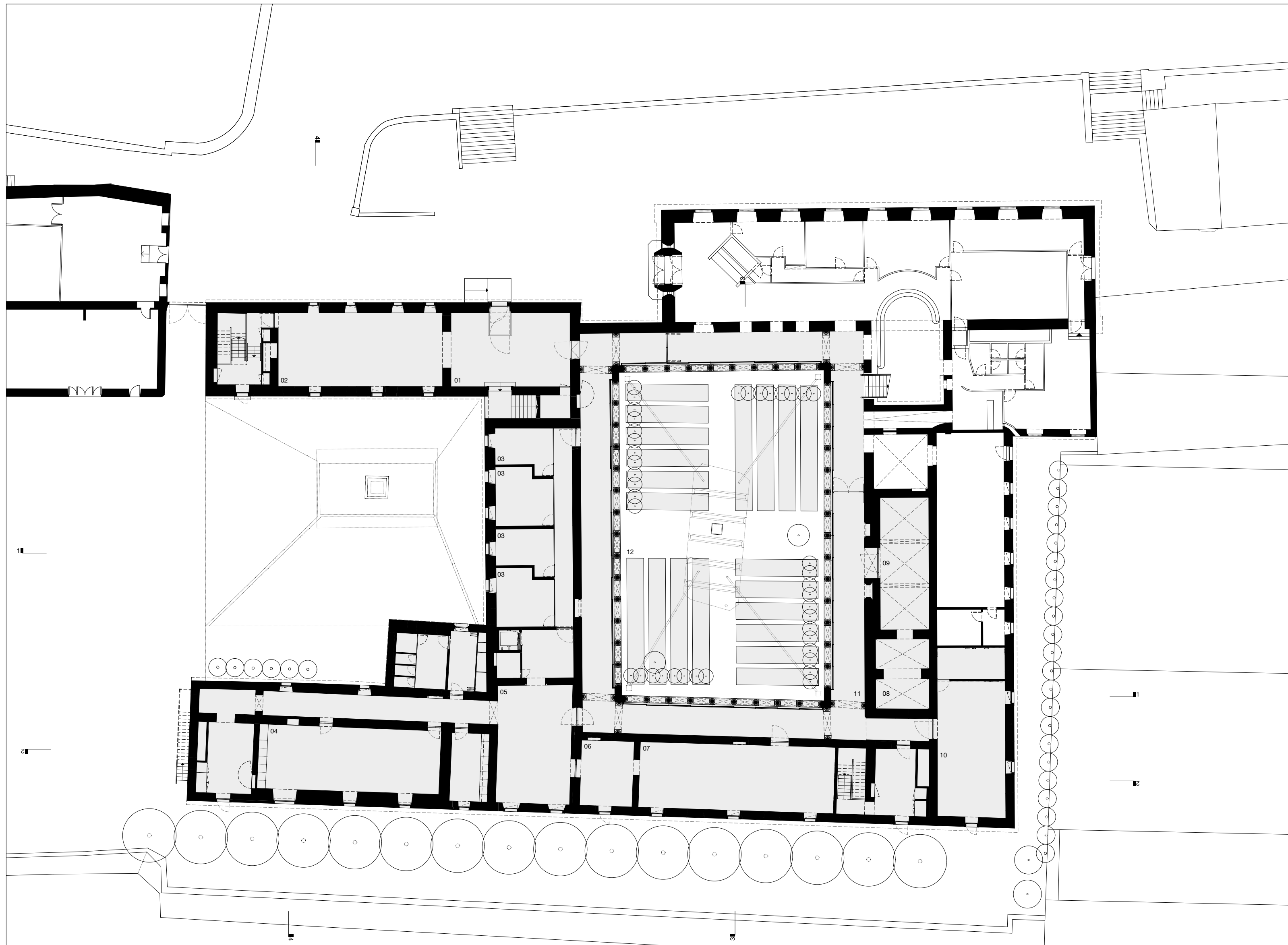
Planta piso 0 — Ground floor plan
