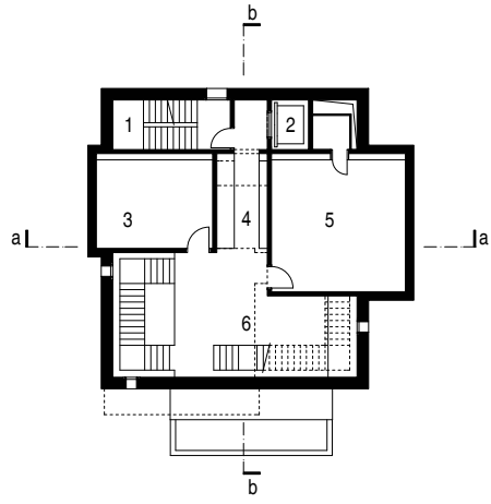
Second floor plan Scale 1:400
